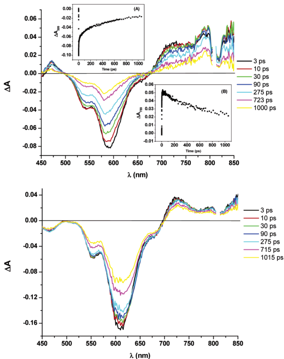
Figure 8. Femtosecond transient spectra of Sq1 (top) and Sq2 (bottom) in dichloromethane; time delays corresponding to frames are given in the spectra ( \lambda_{\text{ex}} = 575 \text{ nm} , 130 fs fwhm). Kinetic profiles of the transient absorbance of Sq1 measured at 599 nm (A) and 789 nm (B) in dichloromethane.
